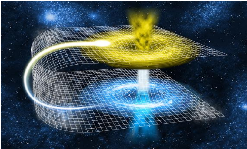
Theory of Wormholes used to travel through Space and Time.
