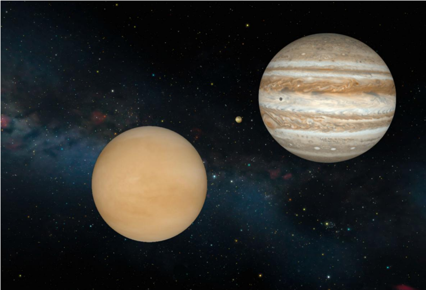
Jupiter-Venus Conjunction in 2015, return of the Christ Stars.
