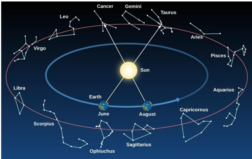
Ecliptic where Sun traverses the primary 12 Signs or Houses.
