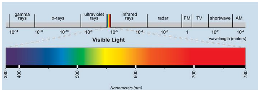
Light Spectrum of the 3 Major Divisions, what See, Feel, Hear.
