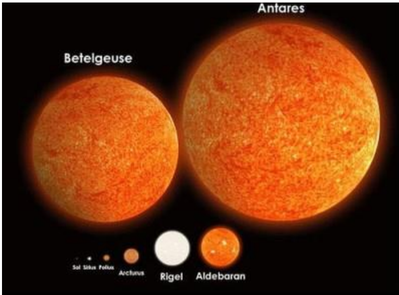
Comparison of Suns as Antares is as big as the Solar System.
